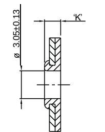
STD-THROUGH HOLE. DETAIL A
